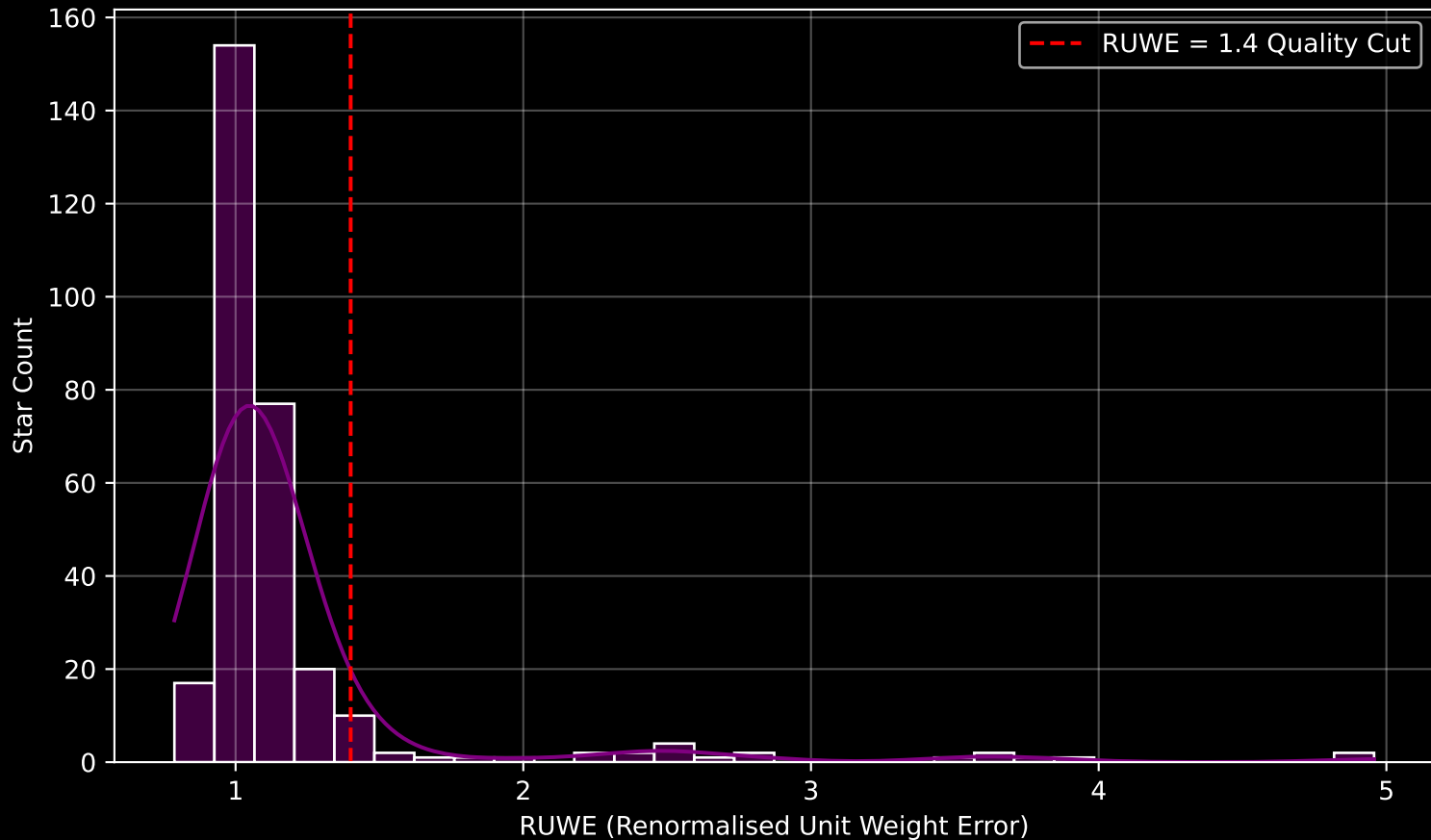
GAPOGEE DR17 Field [173-61] RUWE Distribution (n= 301)
