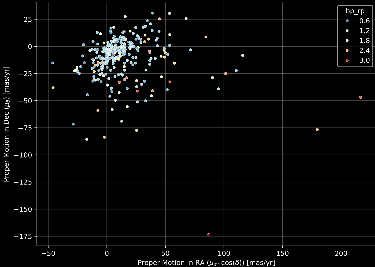
APOGEE DR17 Field: [173-61] Proper Motion Diagram (n= 313)
