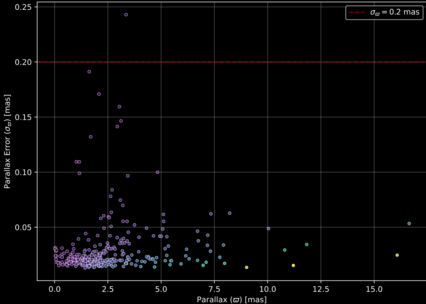
APOGEE DR17 Field: [173-61] Parallax Quality (n= 313)
