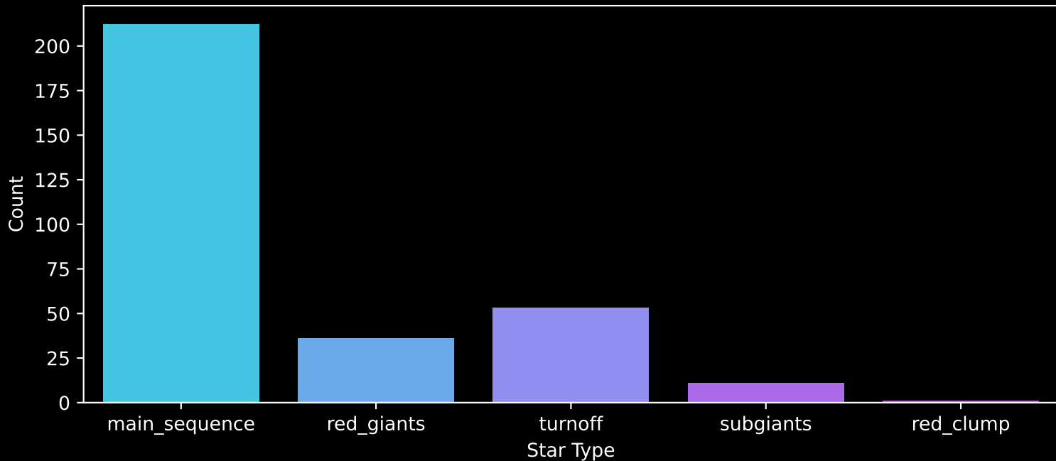
APOGEE DR17 Field: [173-61] Count plot of Star Type
