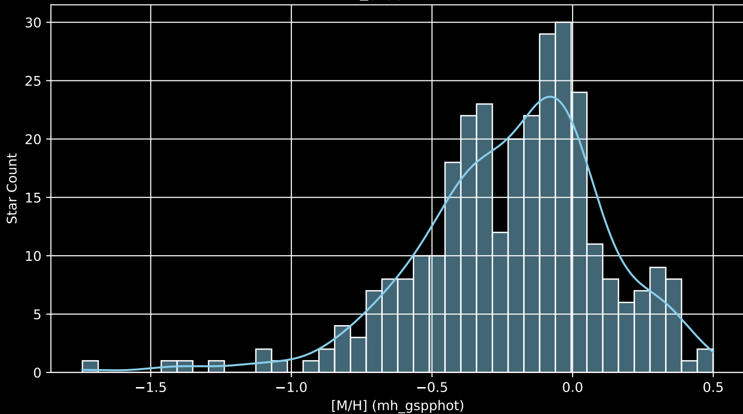
APOGEE DR17 Field: [173-61 [M/H] (mh_gspphot) (n= 312)
