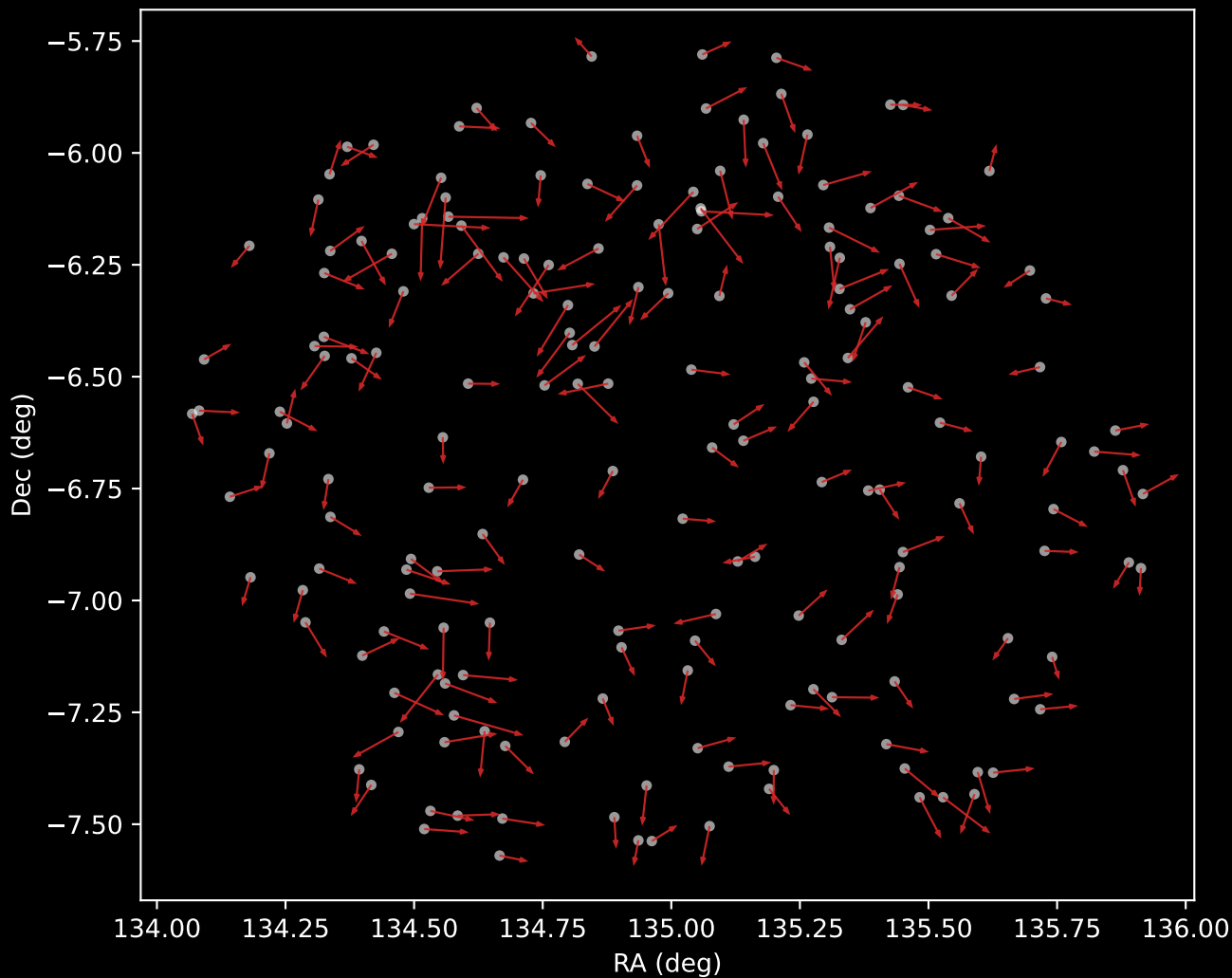
APOGEE DR17 Cluster 6 Proper Motion Vectors (n=186)
